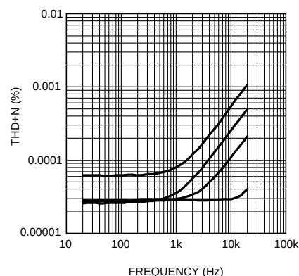
Figure 18. THD+N vs Frequency LME49720/LME49600 headphone amplifier into (from top to bottom at 5kHz): 16Ω at 100mW, 32Ω at 100mW, 64Ω at 150mW, and 300Ω at 30mW ( V_s = \pm 15V , < 10Hz \leq BW \leq 80kHz )
