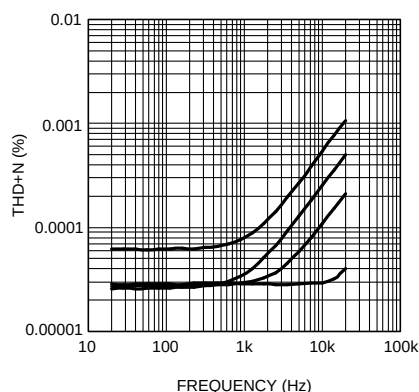
Figure 17. THD+N vs Frequency LME49720/LME49600 headphone amplifier into (from top to bottom at 5kHz): 16Ω at 100mW, 32Ω at 100mW, 64Ω at 35mW, and 300Ω at 8mW ( V_s = \pm 9V , < 10Hz \leq BW \leq 80kHz )
